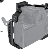
STEP⑤: Locking the left side lock adapter
