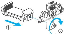
Install the stand for iPad and 15mm LWS support 安装 iPad支架和连接件
